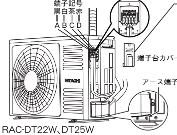
RAC-DT22W, DT25W
