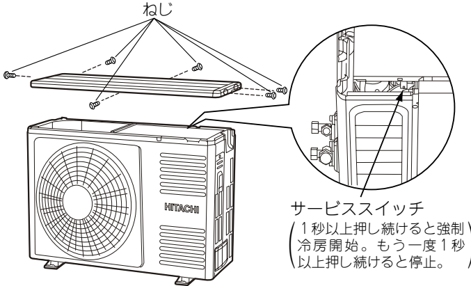
RAC-DT22W、DT25W
