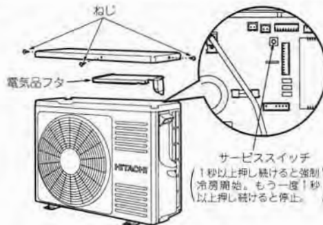
RAC-4000VJ2
